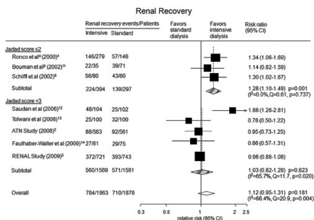
Figure 4. Probability of renal recovery for more intensive versus less intensive RRT regimes. a Two treatment groups (35 and 45 ml/kg per h) were combined for the purpose of analysis. b Two treatment groups (early-low volume and late-low volume) were combined for the purpose of analysis.
